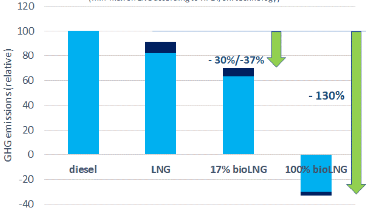
GHG emissions (vehicle + fuel) - 40t LNG truck (min-max on LNG according to HPDI/S.I. technology)
